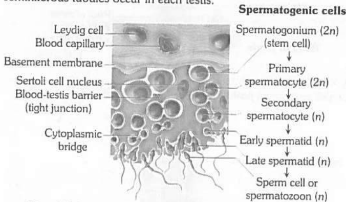
Fig : 6.3-3 T.S. of a seminiferous tubule (diagrammatic)
